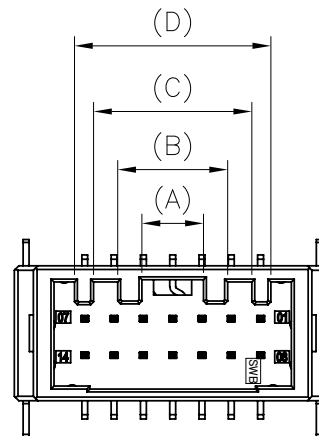
2*07~2*12 Pin
