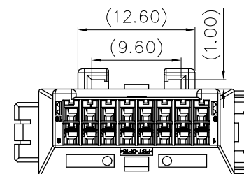
Card slot B 2024AF-2*XXB-PTXX
