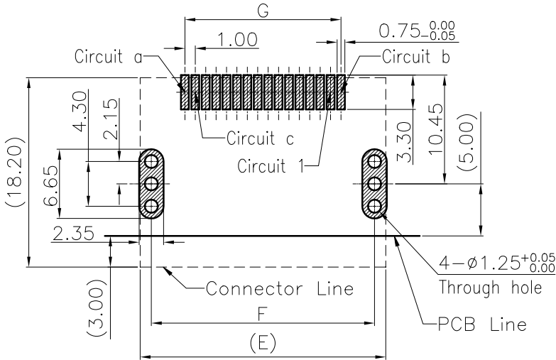
Recommended P.C.B Layout(T=1.6mm) General tolerance \pm 0.05
